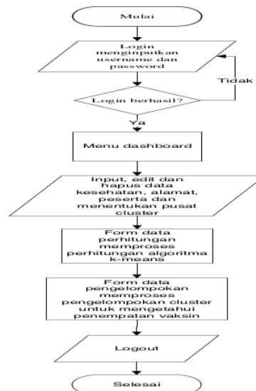
Gambar 3. Flowchart alur sistem
