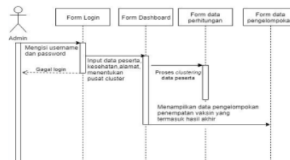
Gambar 6. Sequence Diagram
