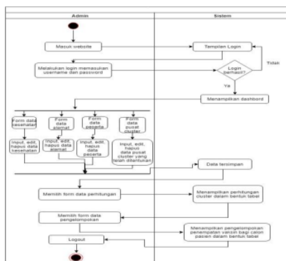
Gambar 5. Activity Diagram
